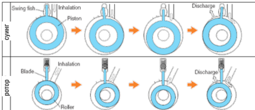
■ Comparison of action between swing compressor and rotary compressor.
