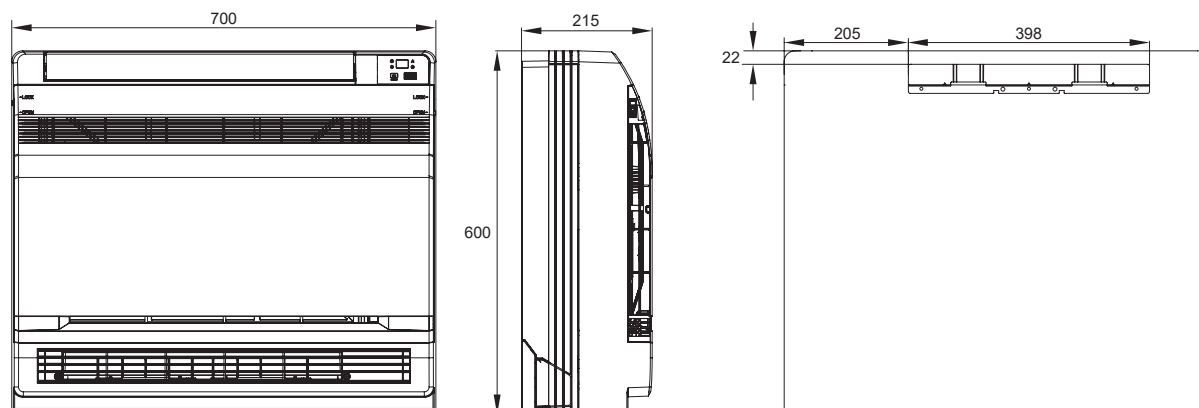
■ GEH09AAXB-K6DNA1A/I - GEH18AAXF-K6DNA1A/I
