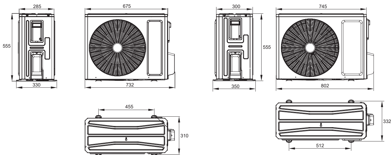
■ GEH09AAXB-K6DNA1A/O
