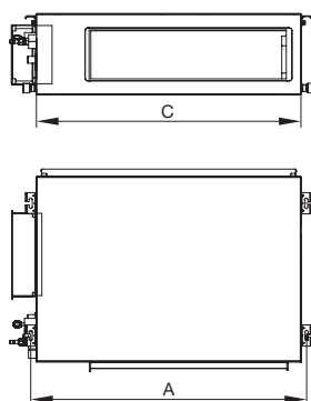
■ GUD35P1/A-S - GUD50PS1/A-S
